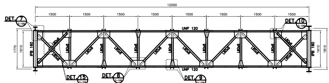
BOTTOM TRUSS ( BRIDGE "3" )
