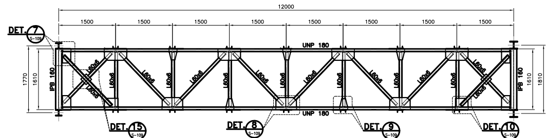
TOP TRUSS ( BRIDGE "3" )
